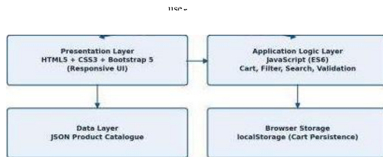
Figure 4.1: System Architecture of ShopEase
